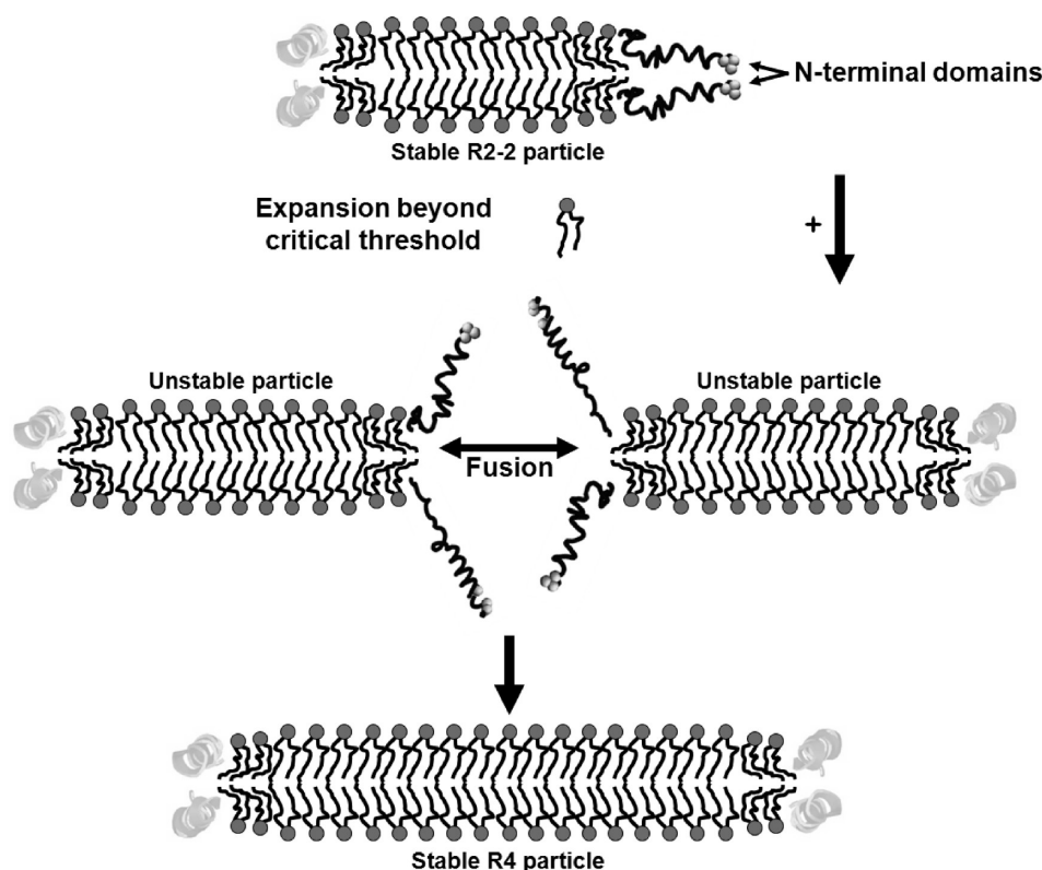
Figure 10. Schematic model of the polar lipid remodeling-switch hypothesis. Postulated role of “sticky” N-terminal proline-rich domains in fusion between particles that have exceeded a critical polar lipid concentration. PL molecules are represented schematically in the usual ball (dark gray) and stick (black) motif. Particles are represented as bilayers in cross section. Central domains (light gray ribbon helices); terminal remodeling-switch domains (dark gray tube helices).
