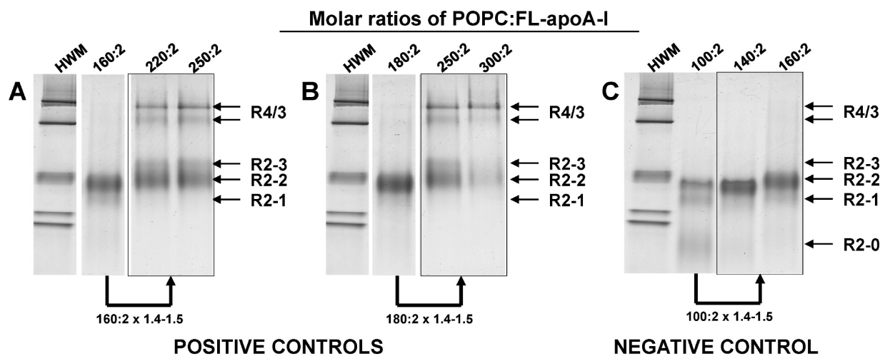
Figure 3. Effects of POPC concentration on particle size distribution of POPC:FL-apoA-I recombinants. The gels (4–20% polyacrylamide) were run for 48 h and stained with colloidal blue. NDGGE of reconstituted particles having POPC:FL-apoA-I molar ratios of (positive controls) (A) 160:2, 220:2, and 250:2 and (B) 180:2, 250:2, and 300:2 and (negative control) (C) 100:2, 140:2, and 160:2. Fusion products are represented by the R4/3 bands.
