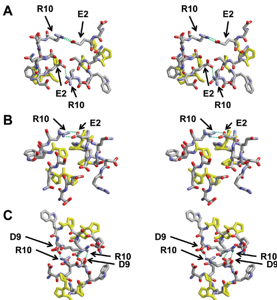
Figure 8. Cross-eyed stereo images in stick CPK representation of intermolecular contacts between overlapping N–N domains, residues 1–10, of three final structures from the R2-2 16 ensemble of 16 MDSA simulations of the 160:24:2 (R2-2) particle. Salt bridges are indicated by dashed green lines. Prolines are in yellow.
