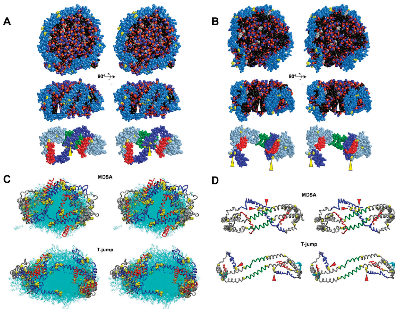
Figure 4. Structural features of one example each of the four MDSA and four 500 K MD T-jump simulations of the 160:24:2 (R2-2) particle. (A) Final structure of one example from the ensemble of four MDSA simulations (R2-2 4 ) of the R2-2 particle. (B) Final structure of one example from the ensemble of four 500 K MD T-jump simulations (X2-2 4 ) of the R2-2 particle. (Upper panel) Cross-eyed stereo image of space-filling models, excluding hydrogens, viewed from the face of the particles with the central domain (helix 5) at the top. (Middle panel) Space-filling models, excluding hydrogens, viewed from the terminal overlap domain side of the particles. Each particle has been rotated 90° from the upper row view as indicated by the arrows. The white arrowheads indicate areas of exposure of acyl chains to solvent. Protein: sky blue except proline (yellow). POPC: phosphorus atoms (gold), phosphate oxygen atoms (red), choline nitrogens and methyls (blue), acyl chains (black). UC: (cpk). (Lower panels) Same view as middle panel showing protein only. Protein: silver blue except proline (yellow), N-terminal domain, residues 1–43 (blue), C-terminal helix 10, residues 220–243 (red), helix 5, residues 121–142 (green). The yellow arrowheads indicate clustering of the N-terminal proline-rich pairs. (C) Cross-eyed stereo images of all the final structures from the ensembles of all four MDSA (R2-2 4 , upper panel) and 500 K MD T-jump (X2-2 4 , lower panel) simulations aligned from residues 77 to 188. POPC and UC are represented in line format (cyan). The protein is represented as a Cα backbone tube model except prolines that are space-filling. The structures are viewed from the terminal overlap domain side of the ensemble particle. N-Terminal domains, residues 1–43 (blue); C-terminal helix 10 domains, residues 220–243, (red); and remainder of protein (gray). (D) Cross-eyed stereo images of average final structures of FL-apoA-I double belt for the four MDSA (R2-2 4 , upper panel) and 500 K MD T-jump (X2-2 4 , lower panel) simulations of the 160:24:2 particle created from calculated average coordinates. The apoA-I double belts are viewed from the helix 5 domain. The protein is represented as a Cα backbone tube model except Cα proline (space-filling yellow). Helix 5 (green), C-terminal helix 10 domains, residues 220–243 (red), N-terminal domains, residues 1–43 (blue), and remainder of protein (gray). The N-terminal (proline-rich) domains are indicated by red arrowheads.
