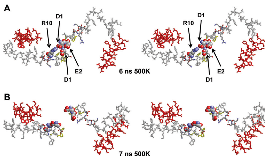
Figure 9. Cross-eyed stick stereo images of the N-terminal interactions of a 240(POPC):36(UC):2(apoA-I) particle subjected to an MD simulation at 310 K for 5 ns and then a T-jump at 500 K for 10 ns. (A) The final molecular interactions holding the N-termini together in the T-jump simulation at 6 ns. (B) The final molecular interactions after separation of the N-termini in the T-jump simulation at 7 ns. The salt bridges between D1 and R10 and E2 and the N-terminal \text{NH}_3 are shown in space-filling CPK representation. N-terminal domain, residues 1–43 (white); C-terminal helix 10, residues 220–243 (red); prolines (yellow).
