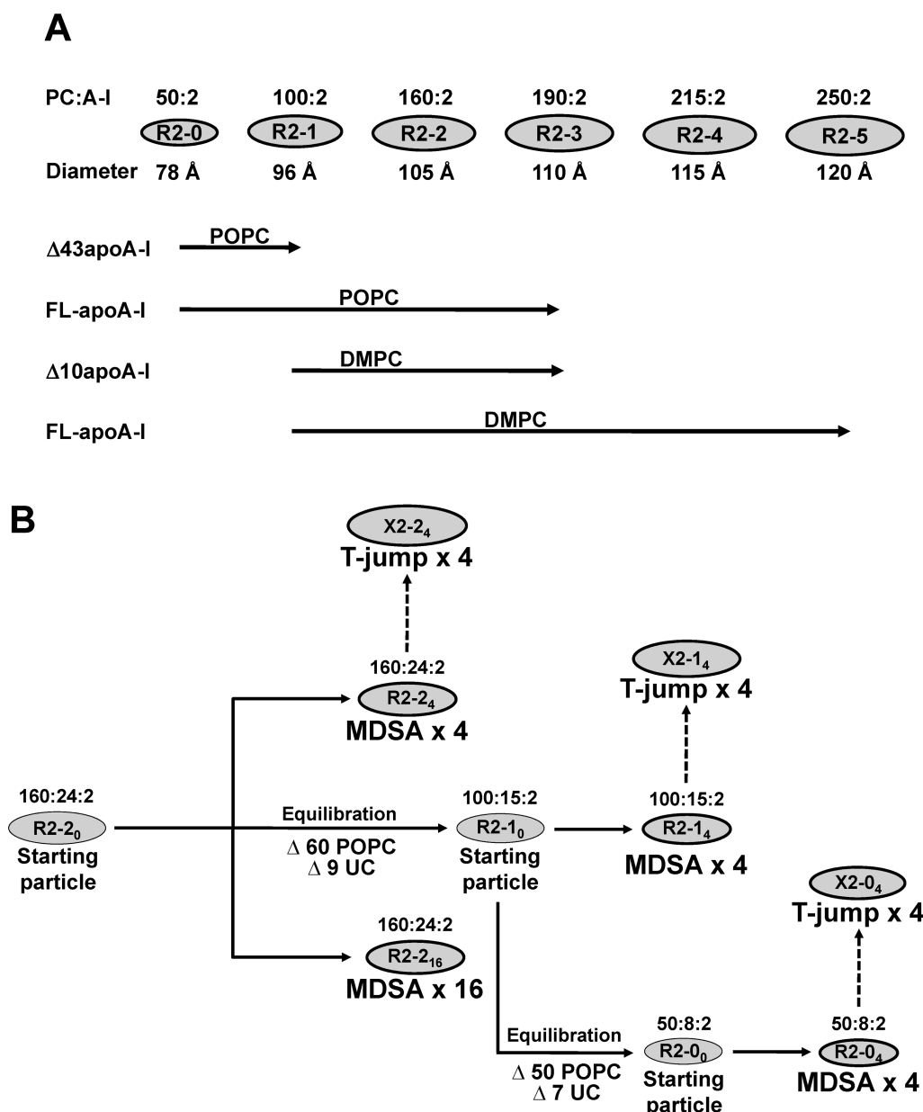
Figure 1. Schematics of the creation, characteristics, and modeling of apoA-I/HDL R2 particles. (A) Schematics of the composition and size of apoA-I/HDL R2 particles. (B) Flow diagram of the creation of the different R2 particles and ensembles by MD, MDSA (30 ns total simulation time), and T-jump (20 ns total simulation time).
