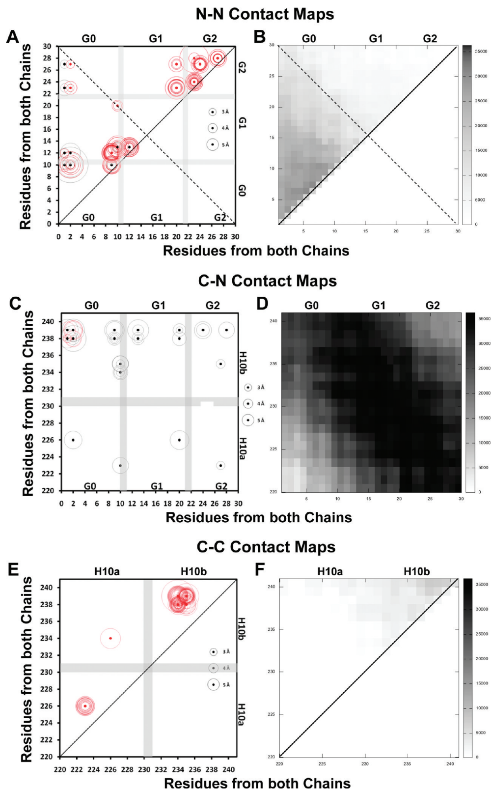
Figure 7. Molecular contact maps between N-terminal pairs, C-terminal pairs, and N-terminal to C-terminal pairs plotted for the R2-2 16 ensemble of 16 MDSA simulations of the 160:24:2 (R2-2) particle. Intermolecular salt bridges are plotted as black dots, intramolecular salt bridges as red dots, and other molecular contacts (fraction of interhelical contacts close enough to allow cross-linking, defined as a C \alpha –C \alpha distance \leq 25 Å, 64 during the last 10 ns of all 16 R2-2 16 MDSA trajectories summed over a total of 20000 frames) as scaled black rectangles (scale to right of plot). Distances of salt bridges are indicated by circles (scaled to right of plot). (A) N–N inter- and intramolecular salt bridges, residues 1–30. (B) N–N intermolecular contacts, residues 1–30. (C) C–C inter- and intramolecular salt bridges, residues 220–241. (D) C–C intermolecular contacts, residues 220–241. (E) C–N inter- and intramolecular salt bridges, residues 1–30 to 220–241. (F) C–N intermolecular contacts, 1–30 to 220–241.
