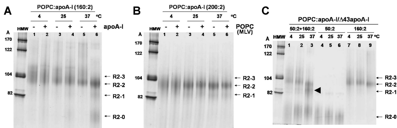
Figure 2. Remodeling of preformed POPC:apoA-I particles by NDGGE analysis. The gels (4–20% polyacrylamide) were run for 48 h and stained with colloidal blue. (A) Preformed POPC:apoA-I complexes at the 160:2 molar ratio were subjected to further incubation for 16 h at 4, 25, or 37 °C without (–) (lane 1, 3, and 5) or with (+) (lane 2, 4, and 6) additional apoA-I to reach a final POPC:apoA-I ratio of 80:2. The results showed that the addition of apoA-I drove the formation of smaller particles with an increase of incubation temperature. (B) Preformed POPC:apoA-I complexes at the 200:2 molar ratio were subjected to further incubation for 16 h at 4, 25, or 37 °C without (–) (lane 1, 3, and 5) or with (+) (lane 2, 4, and 6) additional POPC in the form of MLV to reach a final POPC:apoA-I ratio of 400:2. The results showed that further incubations at increased temperatures sharpened the distribution of POPC:apoA-I assemblies in 16 h, but addition of POPC to preformed assemblies (predominantly R2-2) did not change the size distribution of these particles regardless of incubation temperatures. (C) Preformed R2-0 POPC:Δ43apoA-I particles at a 50:2 ratio and R2-2 POPC:apoA-I particles at a 160:2 ratio were incubated separately (lanes 4–6 and lanes 7–9) or together (lanes 1–3) for an additional 16 h at 4, 25, or 37 °C, respectively. The results showed that a new intermediate-sized particle (R2-1) (solid arrowhead) was formed at the highest incubation temperature.
