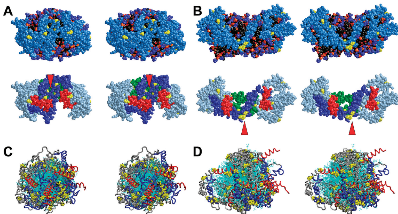
Figure 5. Cross-eyed stereo images of structural features of the four MDSA and four 500 K MD T-jump simulations of the 100:15:2 (R2-1) and 50:8:2 (R2-0) particles. (A) Final structure of one example from the ensemble of four MDSA simulations (R2-1 4 ) of the R2-1 particle. (B) Final structure of one example from the ensemble of four 500 K MD T-jump simulations (X2-1 4 ) of the R2-1 particle. (Top panels) Space-filling models, excluding hydrogens, viewed from the terminal overlap domain side of the particles. Protein: sky blue except proline (yellow). POPC: phosphorus atoms (gold), phosphate oxygen atoms (red), choline nitrogens and methyls (blue), and acyl chains (black). UC: (cpk). (Bottom rows) Same view as top row but showing protein only. Protein: silver blue except proline (yellow), N-terminal domain, residues 1–43 (blue), C-terminal helix 10, residues 220–243 (red), and helix 5, residues 121–142 (green). The red arrowheads indicate clustering of the N-terminal proline-rich pairs. (C) All of the final structures from the ensemble of four R2-0 MDSA simulations (R2-0 4 ) aligned at residues 77–188. (D) All of the final structures from the ensemble of four R2-0 500 K MD T-jump simulations (X2-0 4 ) aligned at residues 77–188. POPC and UC are represented in line format (cyan). The protein is represented as a C \alpha backbone tube model except prolines that are space-filling. The structures are viewed from the terminal overlap domain side of the particle. N-Terminal domains, residues 1–43 (blue); C-terminal helix 10 domains, residues 220–243, (red); and remainder of protein (gray).
