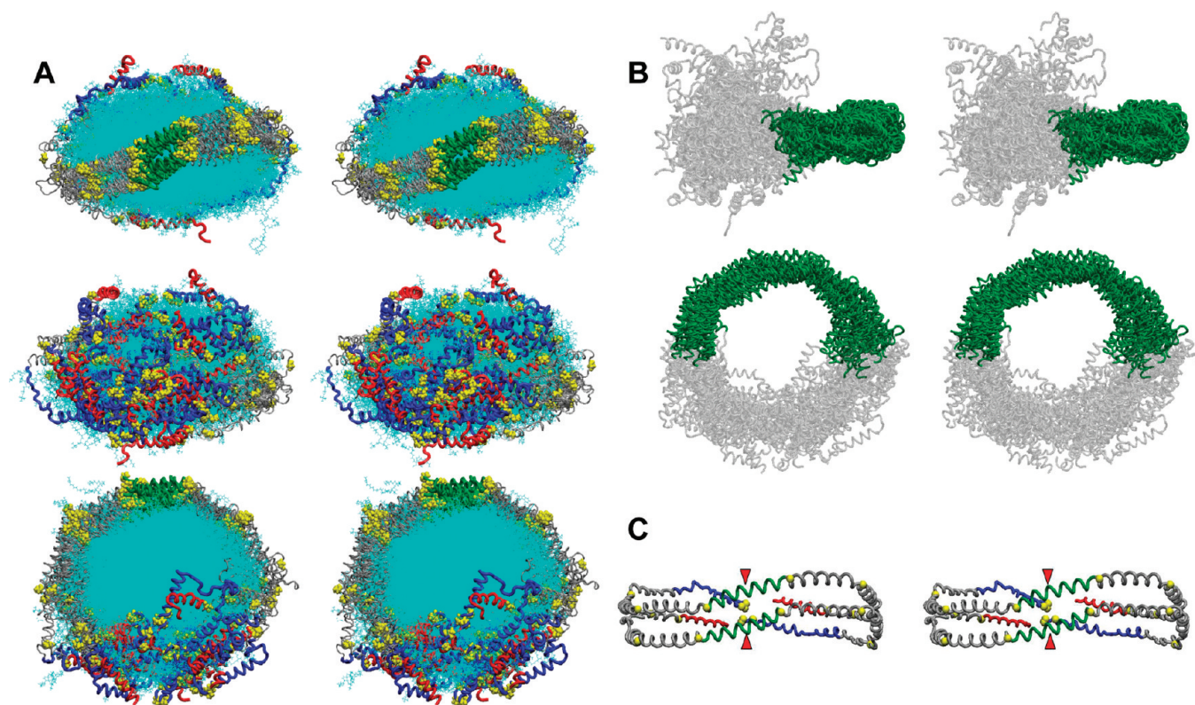
Figure 6. Detailed stereo images of the double belt structure of FL-apoA-I in the R2-2 16 ensemble after MDSA. The protein chains of the final structures of the 16 member ensemble were aligned between residues 77 and 188, the domain containing the interhelical solvent-inaccessible salt bridges. (A) Cross-eyed stereo images of the aligned structures viewed from three different directions. Upper panel, view from helix 5 side; middle panel, view from terminal domain side; lower panel, view from disk top. C-Terminal helix 10 domains, residues 220–243 (red licorice), N-terminal domains, residues 1–43 (blue licorice), helix 5 domain (green licorice), remainder of protein (gray licorice), and lipid (cyan line). (B) Cross-eyed stereo image of the aligned structures showing the relative immobility of the central domain (green licorice) and mobility of the terminal domains (gray licorice). (C) Cross-eyed stereo image of an average final structure created from calculated average coordinates. The apoA-I double belt is viewed from the helix 5 domain. The protein is represented as a C \alpha backbone licorice model except C \alpha proline (space-filling yellow). Helix 5 (green), C-terminal helix 10 domains, residues 220–243 (red), N-terminal domains, residues 1–43 (blue), and remainder of protein (gray). The N-terminal proline-rich domains are indicated by red arrowheads.
